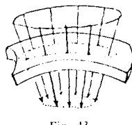
Fig. 43 Light rays are radial when projected through spherical planes
