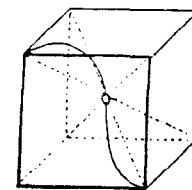
Fig. 47 The six outer mirrors of gravitation
