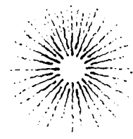
Fig. 6 The explosive action
