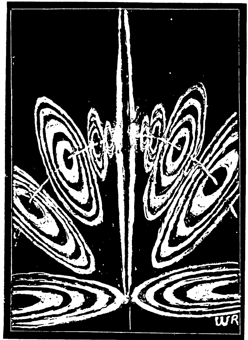
FIG. 64 Compression rings on the wave in octave formation, which is the basic cause of this curved universe of motion. In the center of this diagram are the expansion rings and spiral arms which radiate the heat which the cold has generated. (See our new Laws of Thermodynamics)
