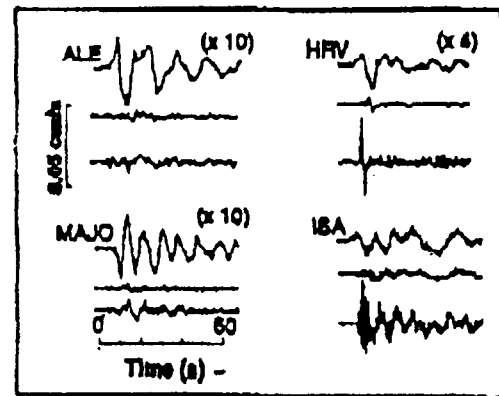
Fig. 4. Broad-band velocity records from four stations (ALE: epicentral distance A = 5185 km azimuth = 9^\circ ; HRV: A = 4366 km, azimuth = 69^\circ ; MAJO: A = 8029 km azimuth = 306^\circ ; ISA: A = 745 km azimuth = 132^\circ ) for the main shock (top trace) and the first (middle) and second (lower) aftershocks. The amplitudes of the seismograms at ALE, HRV and MAJO are increased relative to ISA for display. The large amplitudes of the second aftershock relative to the other two events in the long-strike azimuth (ISA) is attributable to rupture directivity.
