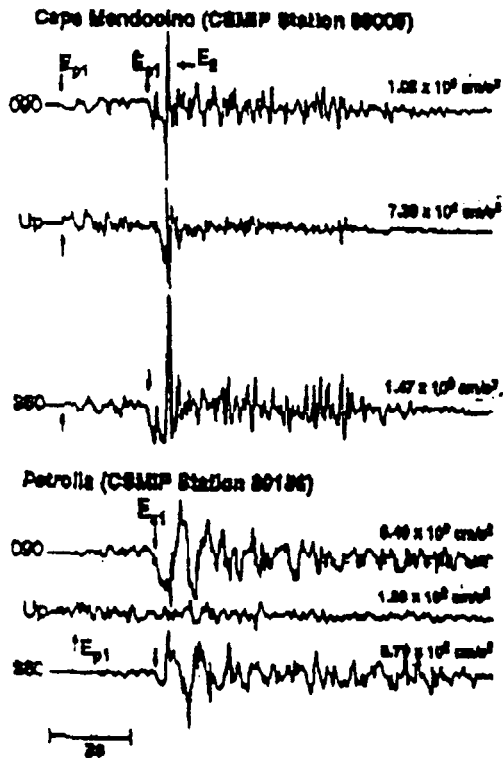
Fig. 5. Strong-motion recordings and peak accelerations on three axes from stations of the California Strong Motion Instrumentation Program (CSMIP) at Cape Mendocino and Petrolia (22). Discernible first-motion-directions of the P and S waves for long-period event ( E_{p1} and E_{g1} ) are indicated, as is the large, high-frequency pulse at Cape Mendocino ( E_2 ).
