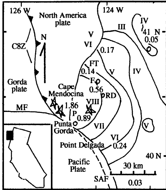
Fig. 1. Simplified tectonic map in the vicinity of the Cape Mendocino earthquake sequence. Stars, epicenters of three largest earthquakes contours. Modified Mercalli intensities (values Roman numerals) of main shock; open circles strong motion instrument sites (22) (adjacent numbers give peak horizontal accelerations in g). Abbreviations: FT, Fortuna; F, Ferndale; RD, Rio Dell; S, Scotia; P, Petrolia; H, Honeydew, MF, Mandocino fault; CSZ seaward edge of Cascadia subduction zone; SAF, San Andreas fault.
