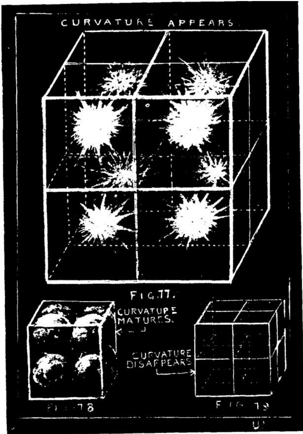
The outward pressures of radiation and centrifugal force lose all spherical form and curvature by disappearance into the six planes of zero curvature, which bound all cubic wave-fields.
