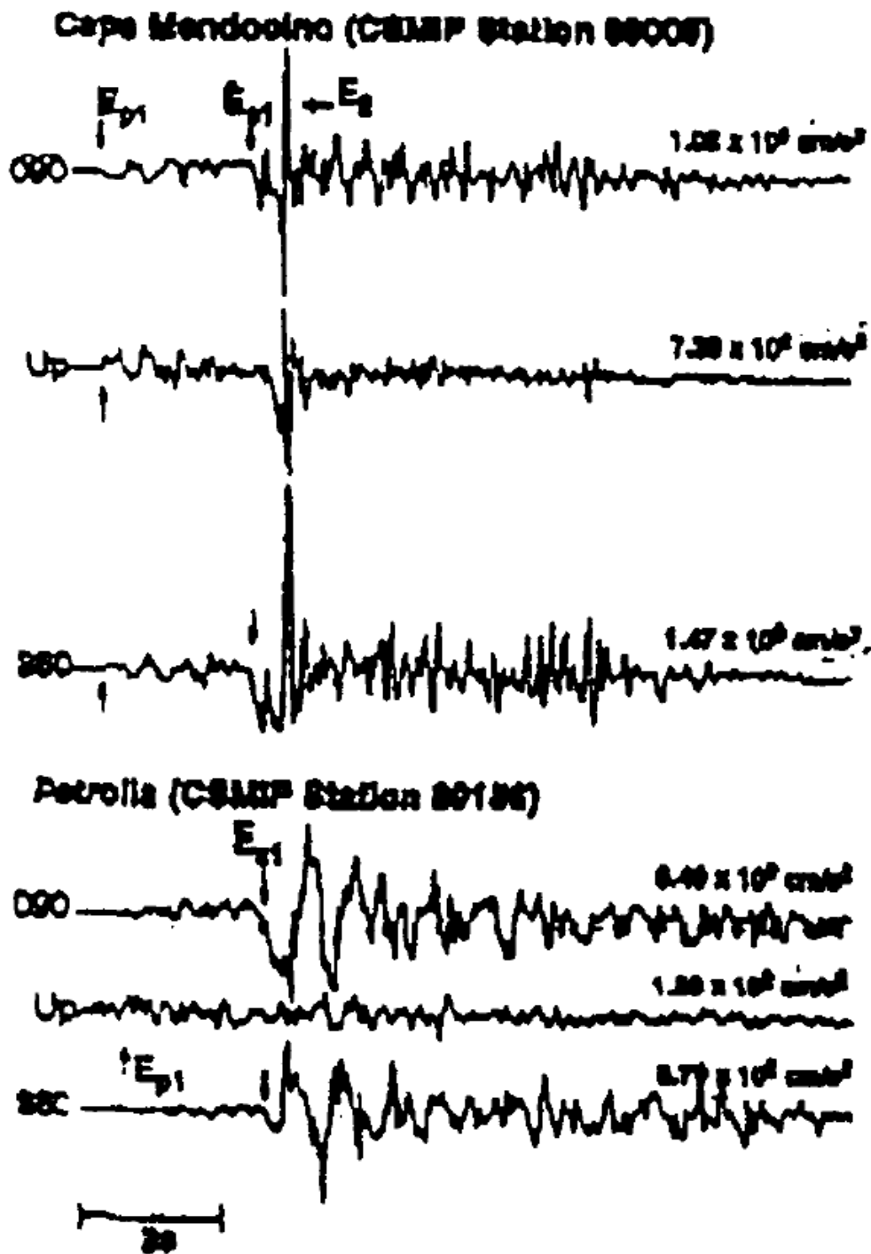
Fig. 5. Strong-motion recordings and peak accelerations on three axes from stations of the California Strong Motion Instrumentation Program (CSMIP) at Cape Mendocino and Petrolia (22). Discernible first-motion-directions of the P and S waves for long-period event ( E_{p1} and E_{g1} ) are indicated, as is the large, high-frequency pulse at Cape Mendocino ( E_2 ).
