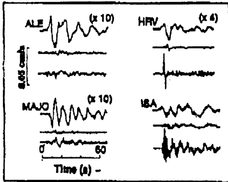
Fig. 4. Broad-band velocity records from four stations (ALE: epicentral distance A = 5185 km azimuth = 9^\circ ; HRV: A = 4366 km, azimuth = 69^\circ ; MAJO: A = 8029 km azimuth = 306^\circ ; ISA: A = 745 km azimuth = 132^\circ ) for the main shock (top trace) and the first (middle) and second (lower) aftershocks. The amplitudes of the seismograms at ALE, HRV and MAJO are increased relative to ISA for display. The large amplitudes of the second aftershock relative to the other two events in the long-strike azimuth (ISA) is attributable to rupture directivity.
